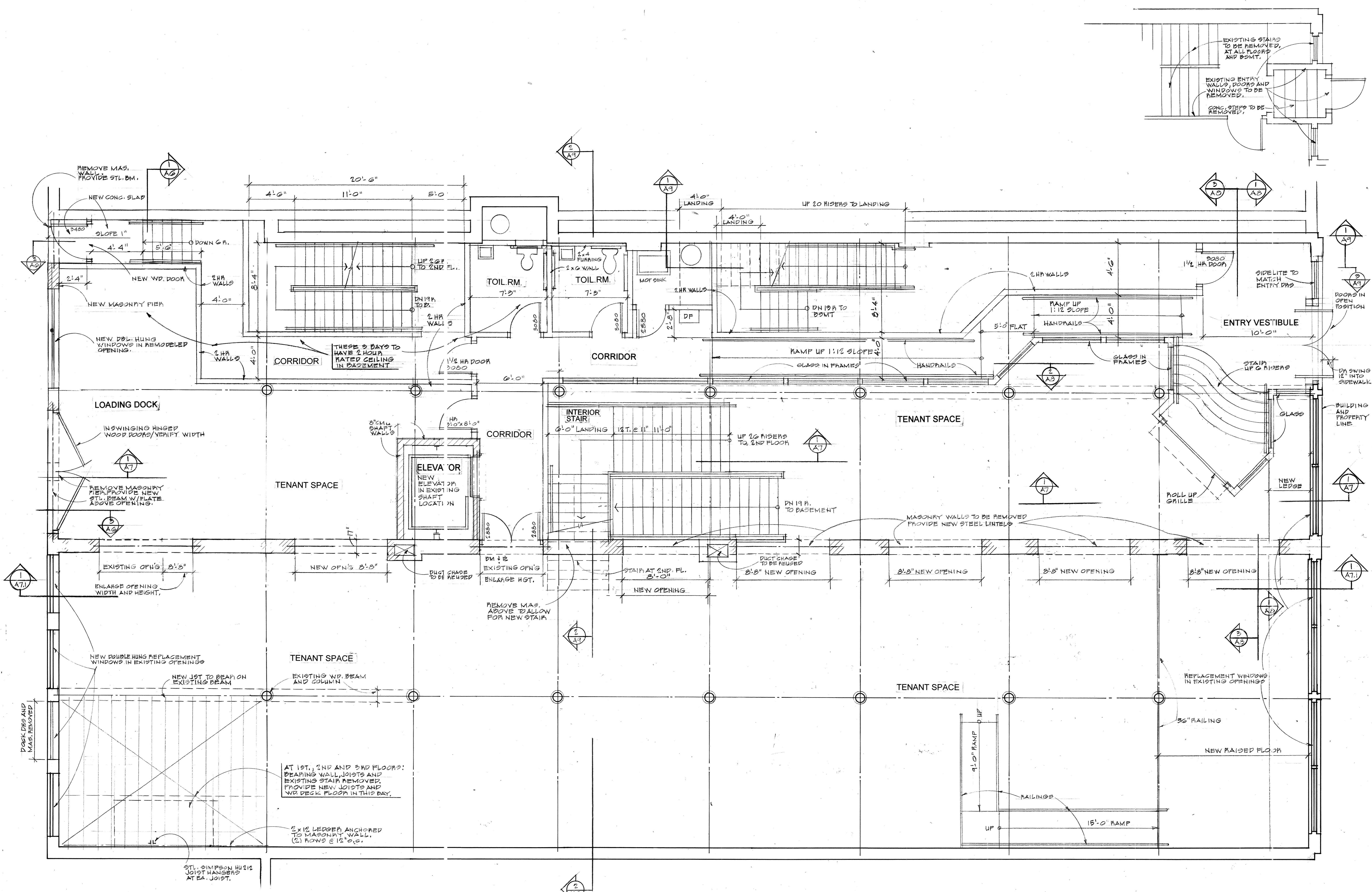
1 A2 FIRST FLOOR PLAN SCALE 1/4"=1'-0"
