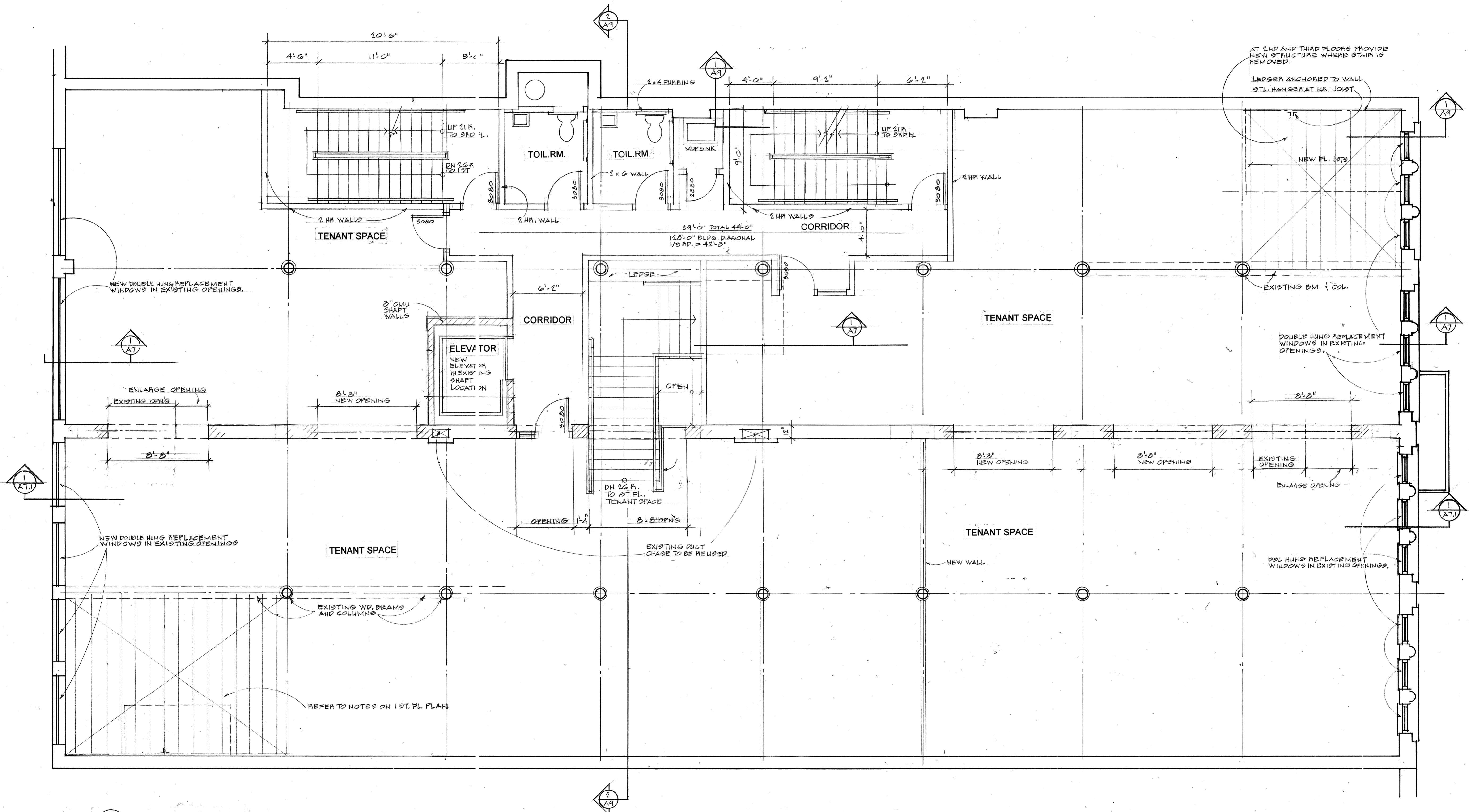
1 SECOND FLOOR PLAN A3 SCALE: 1/4"=1'-0"
